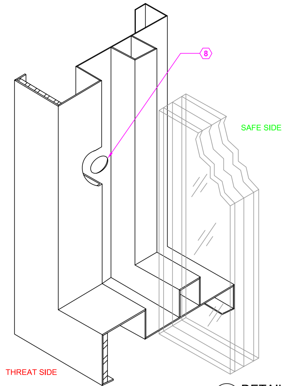
3 DETAIL: 3D BLOW-UP SCALE: NOT TO SCALE
