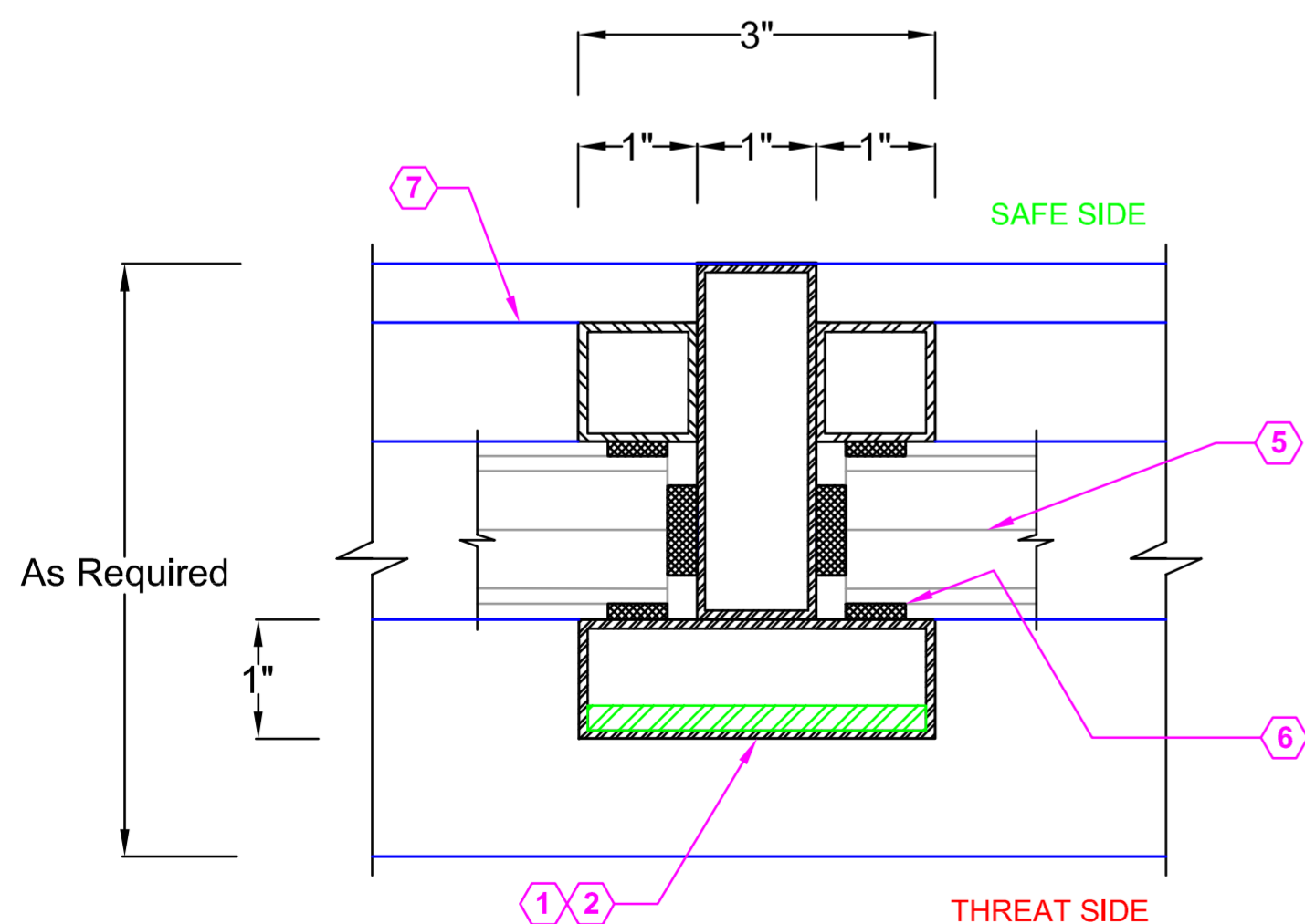
1 DETAIL: WINDOW MULLION SCALE: NOT TO SCALE
