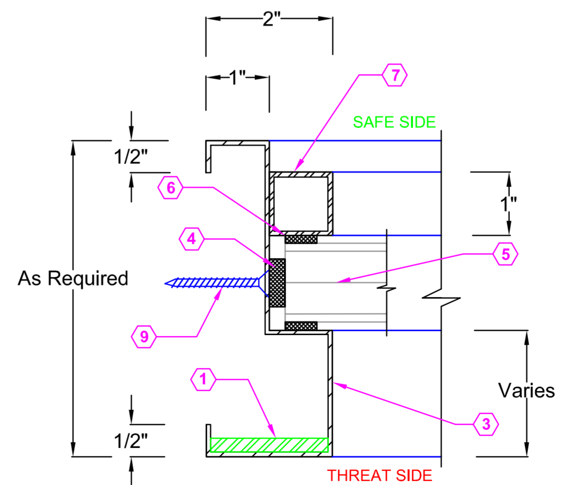
2 DETAIL: WINDOW FRAME SCALE: NOT TO SCALE
